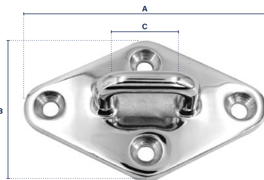
DIAMOND PAD EYE
